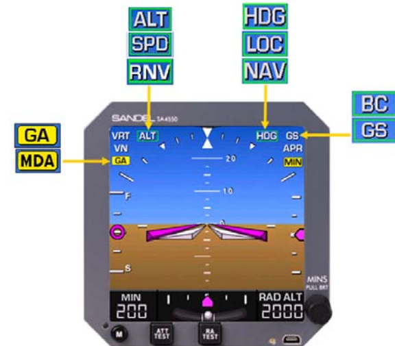
Figure 2-7 Annunciator Locations
