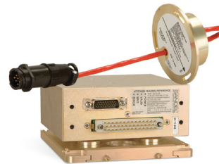
SG102 AHRS
