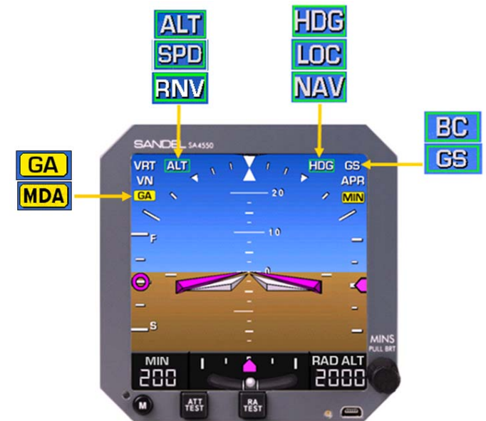
Figure 2-7 Annunciator Locations
